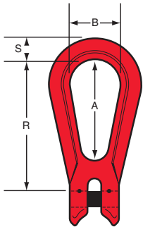
Crosby® Trawlex® Egg Link KSS
